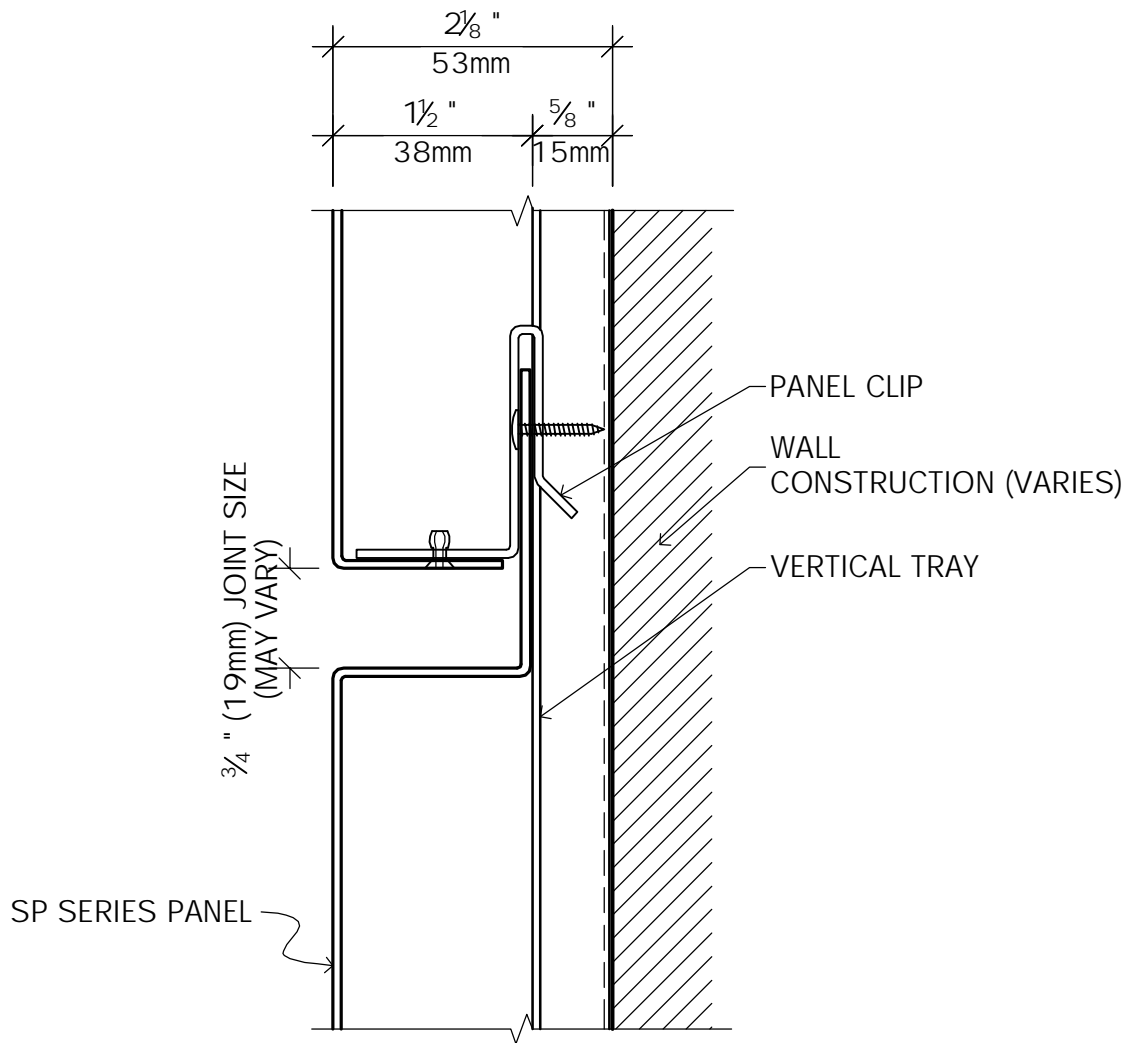
HORIZONTAL JOINT DETAIL
