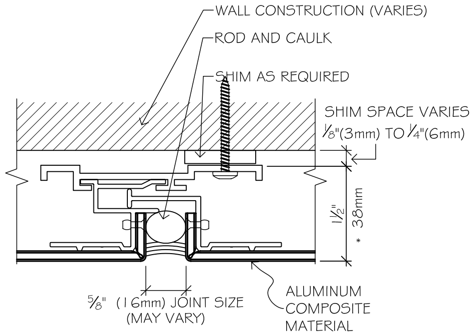
VERTICAL JOINT DETAIL
