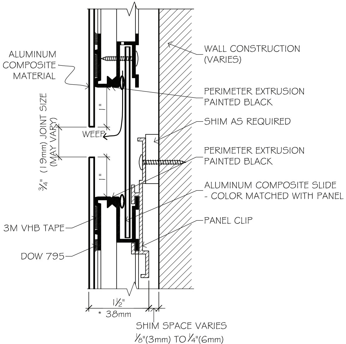
HORIZONTAL JOINT DETAIL
