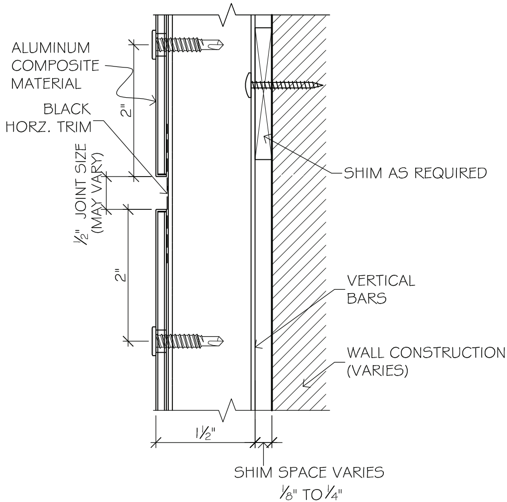
HORIZONTAL JOINT DETAIL
