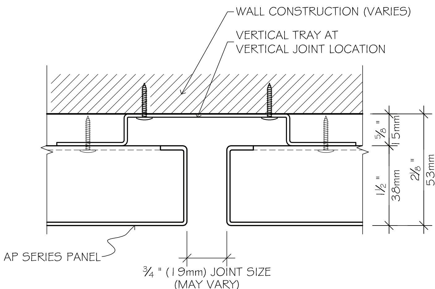
VERTICAL JOINT DETAIL
