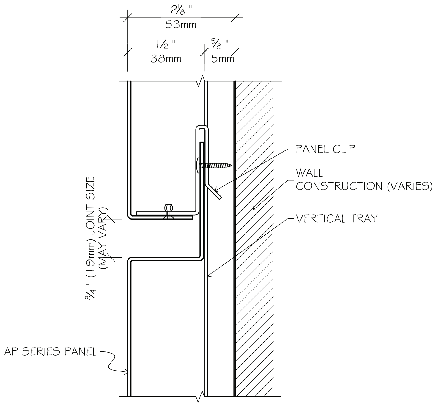
HORIZONTAL JOINT DETAIL
